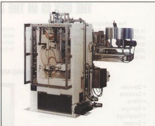
Model 70LCM equipped with screw cap applicator. This is a military version for in-field use.
